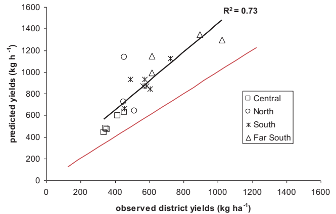
Fig. 3. Relationship between simulated average sorghum yield at specific sites and associated average district yield for sites within central, northern, southern and far-south production zones, respectively.
